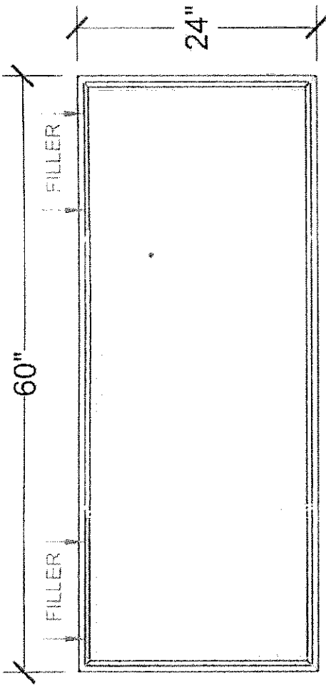
PANEL AND BASE MOLDING LAYOUT
